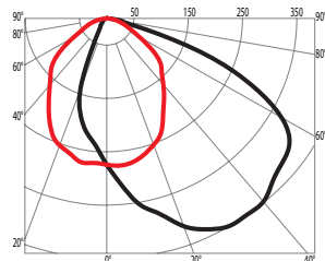
DE-42 HCl-TS 70W - \alpha=0^\circ — 0.0 - 180.0 — 90.0 - 270.0
