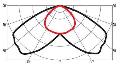
DE-72 HQI-TS 250W - \alpha = 0^\circ - 0.0 - 180.0 - 90.0 - 270.0
