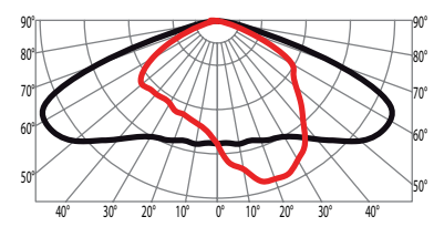
DE-90 SHP-T 150W - \alpha = 0^\circ - 0.0 - 180.0 - 90.0 - 270.0
