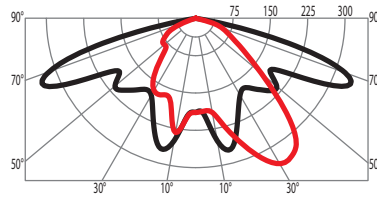
DE-86 CPO-T 140W - \alpha = 0^\circ - 0.0 - 180.0 - 90.0 - 270.0
