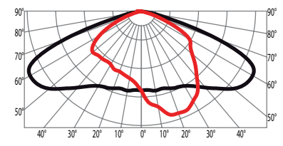
DE-90 SHP-T 150W - \alpha = 0^\circ - 0.0 - 180.0 - 90.0 - 270.0
