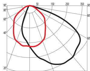
DE-42 HCI-TS 70W - \alpha=0^\circ — 0.0 - 180.0 — 90.0 - 270.0
