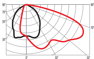
DE-41 HCI-TS 70W - \alpha=0^\circ — 0.0 - 180.0 — 90.0 - 270.0
