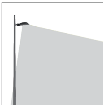
DE-42 HCI-TS 70W - \alpha=0^\circ — 0.0 - 180.0 — 90.0 - 270.0
